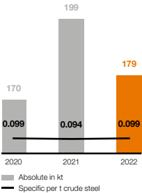
Scope 1 CO 2 emissions of all melt shops in kt / in t per t of crude steel
