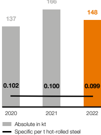
Scope 1 CO 2 emissions of all rolling mills in kt / in t per t of hot-rolled steel
